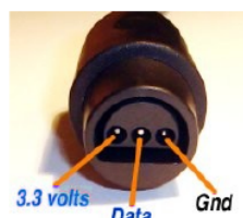
N64 socket pinout (or looking into console)
